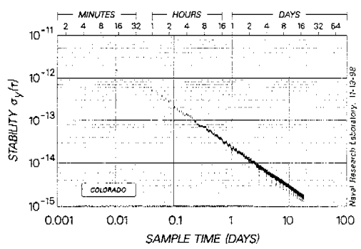
Figure 21. Frequency Stability of Monitor Station Time Reference with Respect to DoD Master Clock via Common-View Time Transfer 1 April 1998 to 1 October 1998
