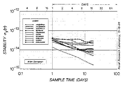
Figure 23. Frequency Stability Profile Comparison of Time References with Respect to DoD Master Clock via Linked Common-View Time Transfer 1 April 1998 to 1 October 1998
